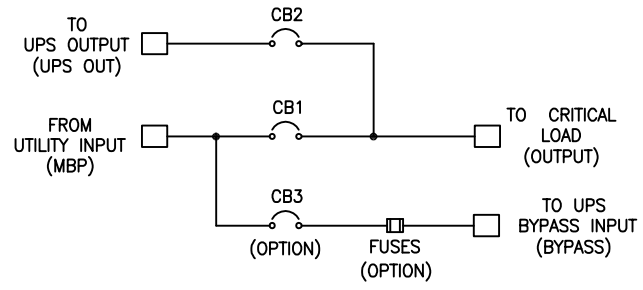
SINGLE LINE DIAGRAM TEXT IN PARENTHESIS REFERS TO TERMINAL LABEL
