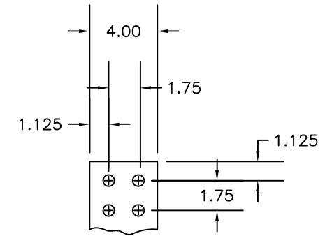
BUSBAR CONNECTION (DETAIL A)
