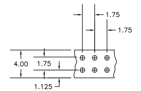
NEUTRAL & GROUND CONNECTION (DETAIL B)
