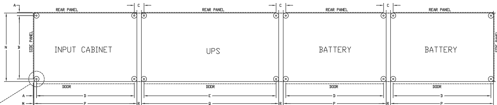
ADJACENT BATTERY CABINETS (STAND-ALONE VERSION NOT SHOWN)
