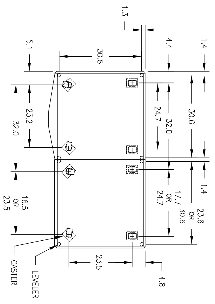
CASTER & LEVELER LOCATIONS
